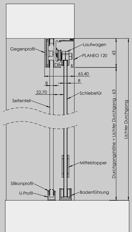
PLANEО 120, DECKENMONTAGE FÜR GLASANLAGEN CEILING MOUNTING FOR GLASS DOOR SYSTEM
